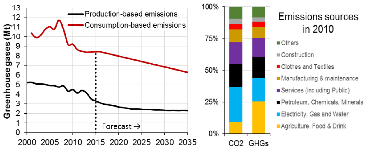
Figure 2: consumption-based emissions trajectories for the area's total consumption-based, and production-based emissions.
